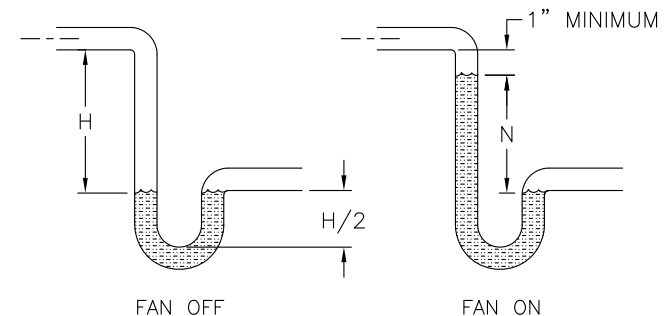
NEGATIVE PRESSURE TRAP* (DRAW THRU FAN)
